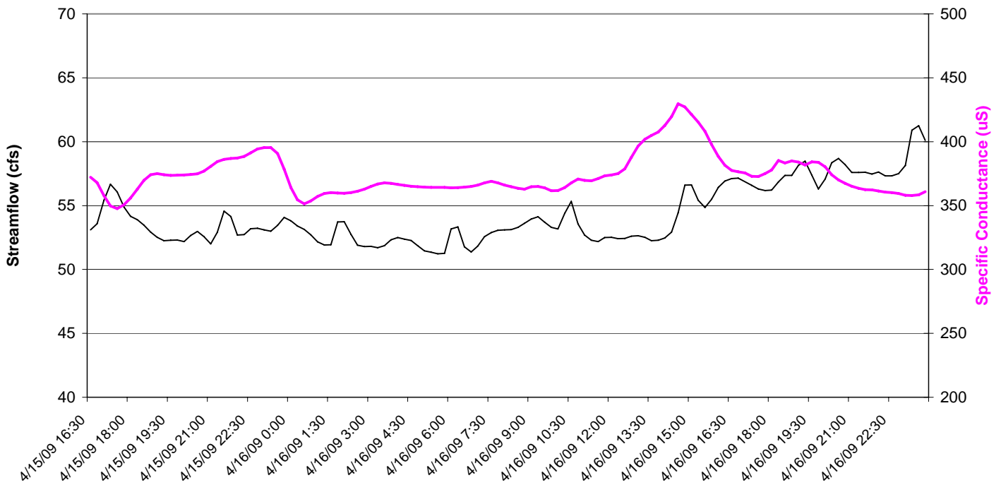
Clear Creek CC-40 Flow and Conductance April 15, 2009 Big 5 Event
