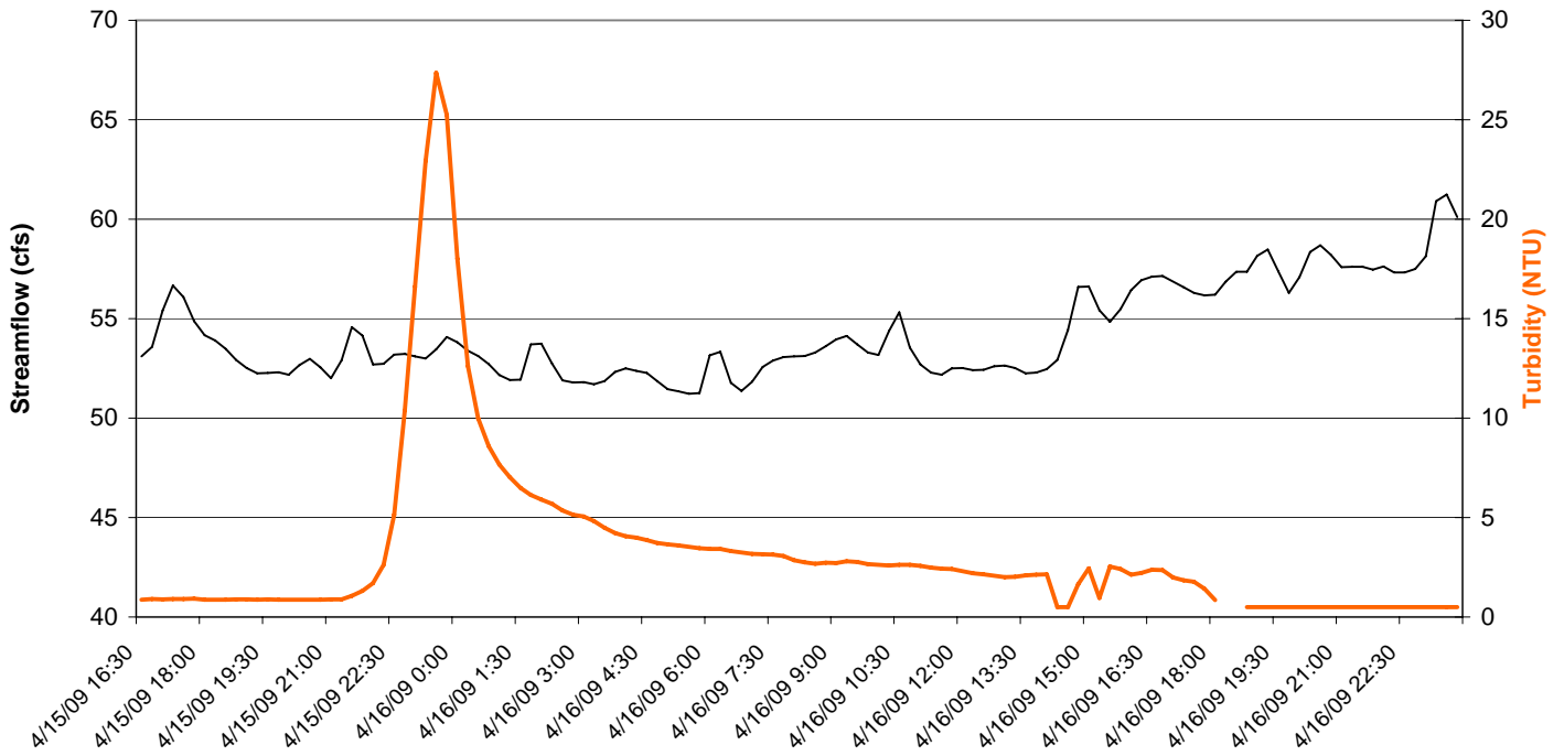
Clear Creek CC-40 Flow and Turbidity April 15, 2009 Big 5 Event
