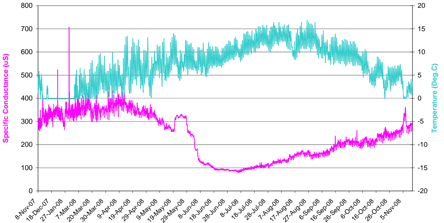
Clear Creek above Johnson Gulch near Kermitts (CC-40) Specific Conductance and Temperature: November 2007 to November 2008
