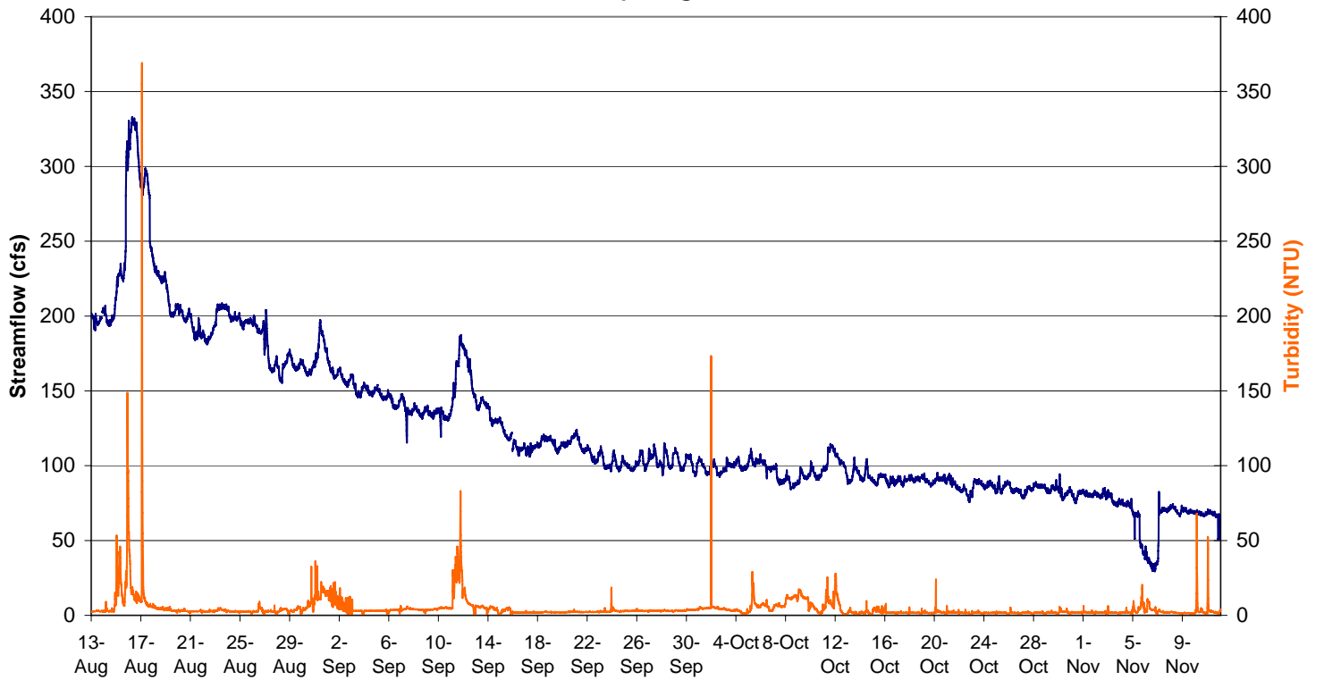
Clear Creek above Johnson Gulch near Kermitts (CC-40) Streamflow and Turbidity: August to November 2008
