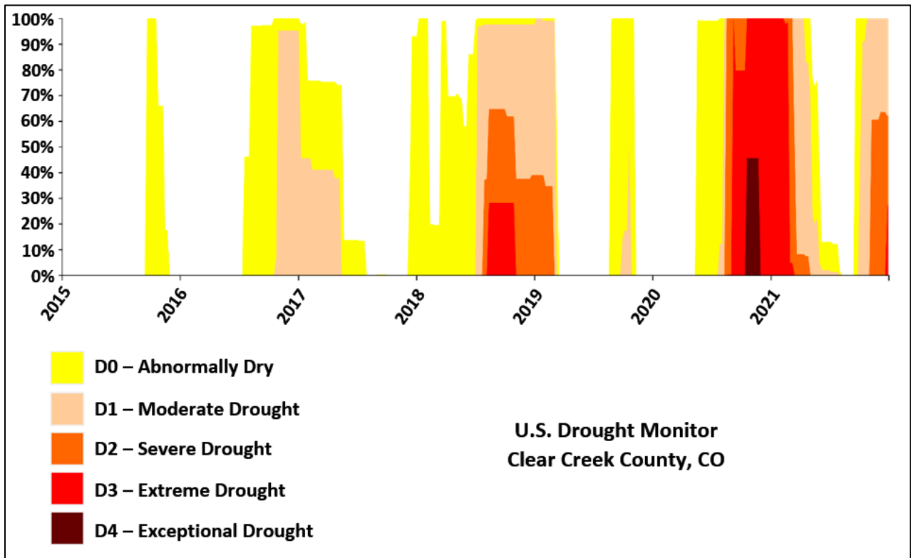
Figure 6. U.S. Drought Monitor History for 2015 - 2021 2
